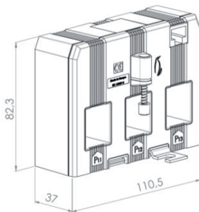
ASKDS 25
