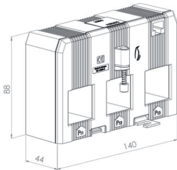
ASKDS 33
